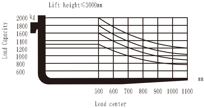
Load chart
